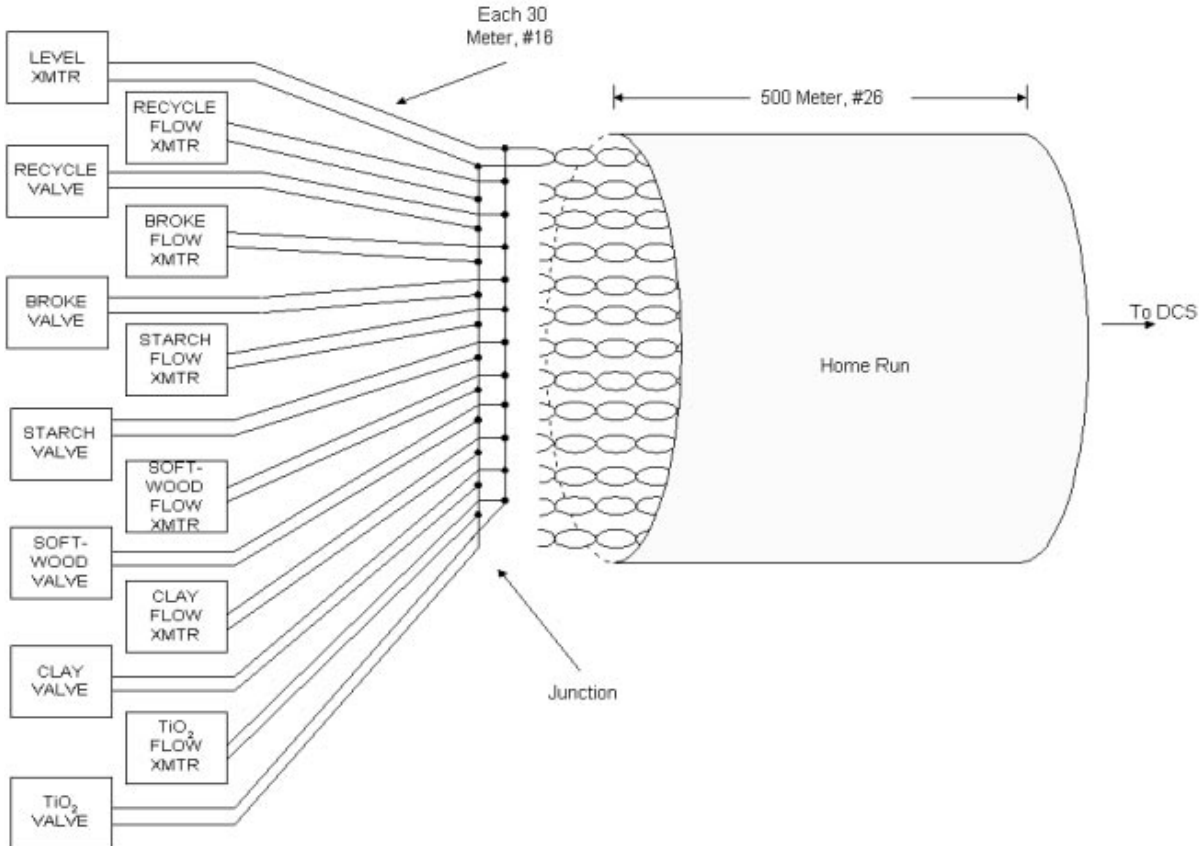
Figure 7.2-4 Proposed Fieldbus Wiring for Paper Mill
