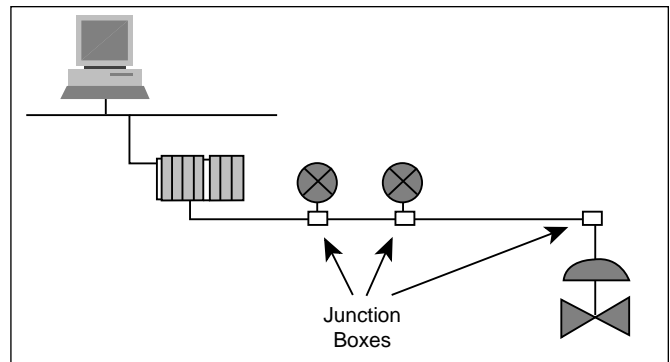
Figure 5.2-1 Bus with Spurs Topology
