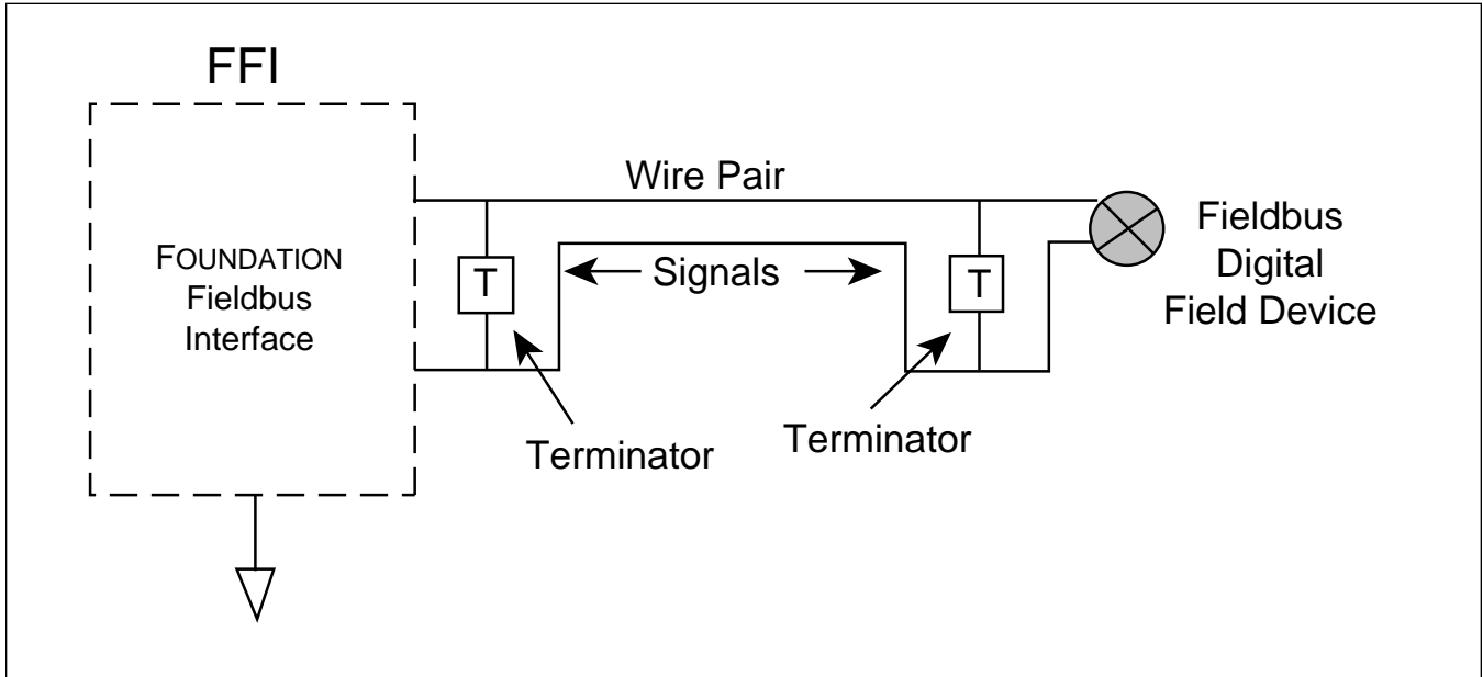
Figure 4.1-2 Simple Fieldbus Network
