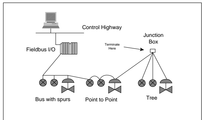
Figure 5.5-1 Mixed Topology
