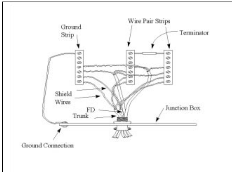
Figure 4.6-3 Field Instrument Wiring Junction
