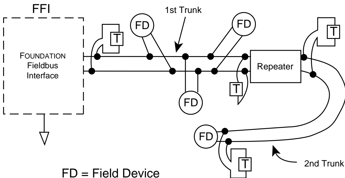
Figure 4.4-1 Adding a Repeater to the Network
