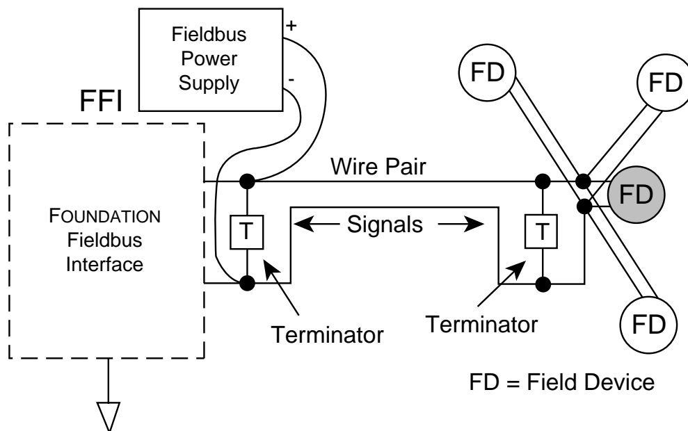
Figure 4.8-1 Adding a Power Supply to the Network
