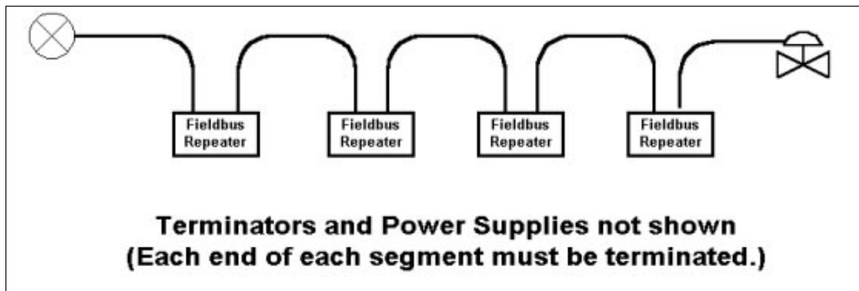
Figure 6.10-1 Maximum Use of Fieldbus Repeaters
