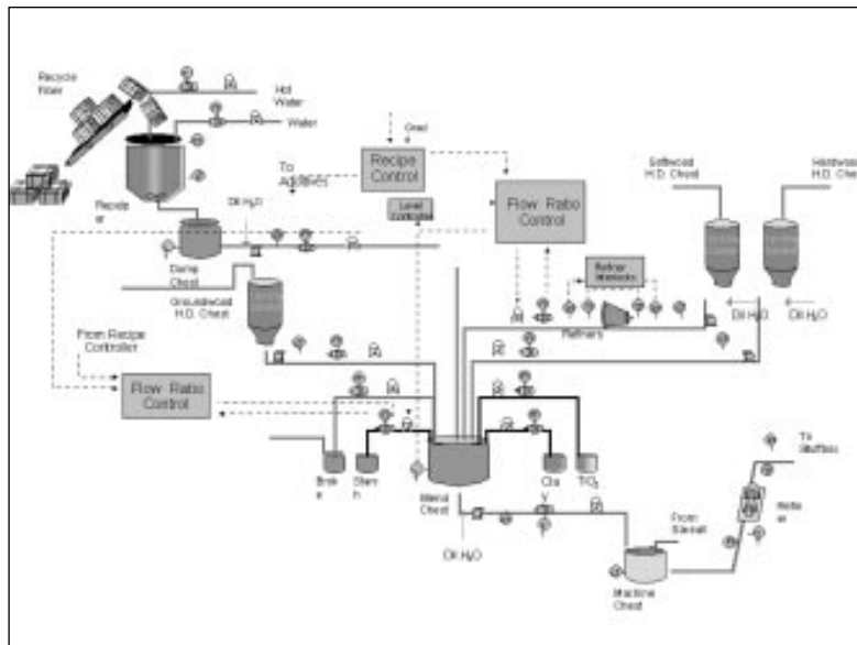
Figure 7.2-2 P & ID Diagram of Typical Paper Mill Example
