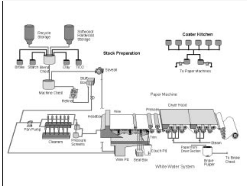
Figure 7.2-1 Diagram of Typical Paper Mill
