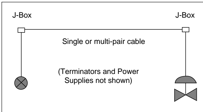
Figure 5.1-1 Simple Point-to-Point Topology
