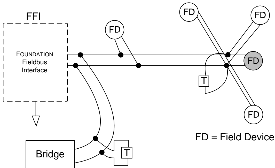
Figure 4.2-1 Addition of a Device and a Bridge to Fieldbus Network
