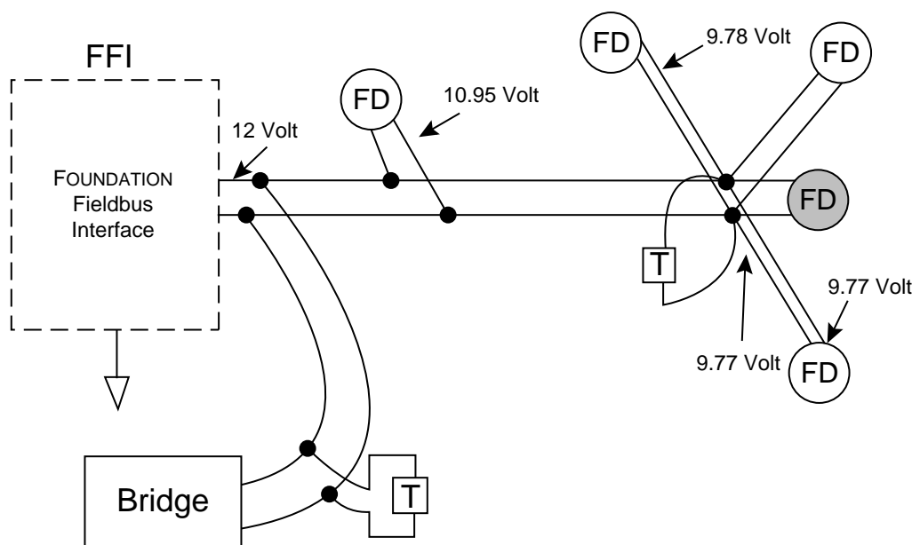
Figure 4.8-2 Voltages at Network Powered Devices
