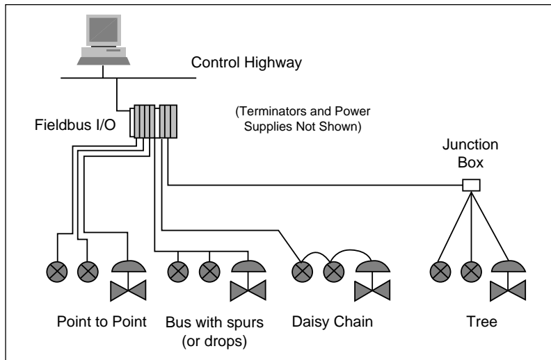
Figure 5.0-1 Possible Fieldbus Topologies
