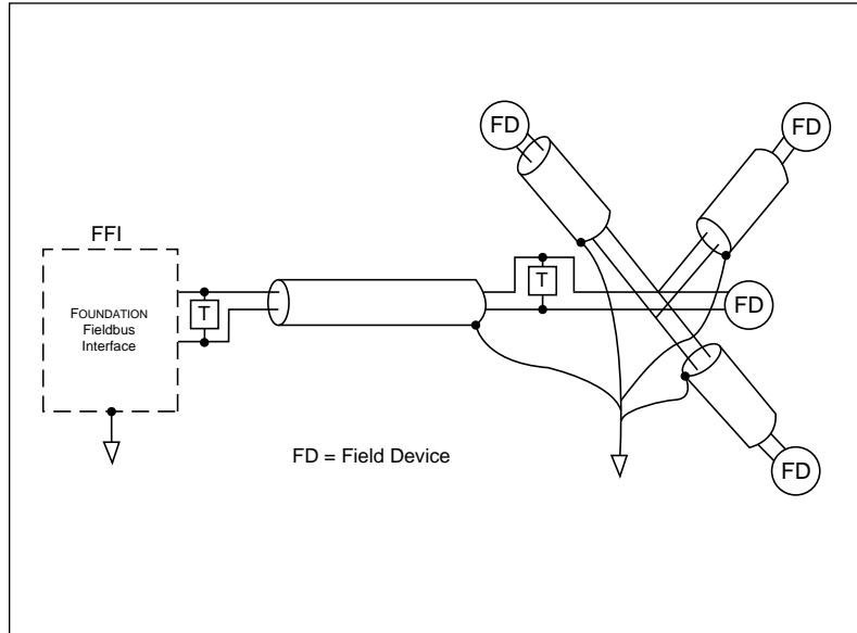
Figure 4.6-2 Use of Shielded Cable
