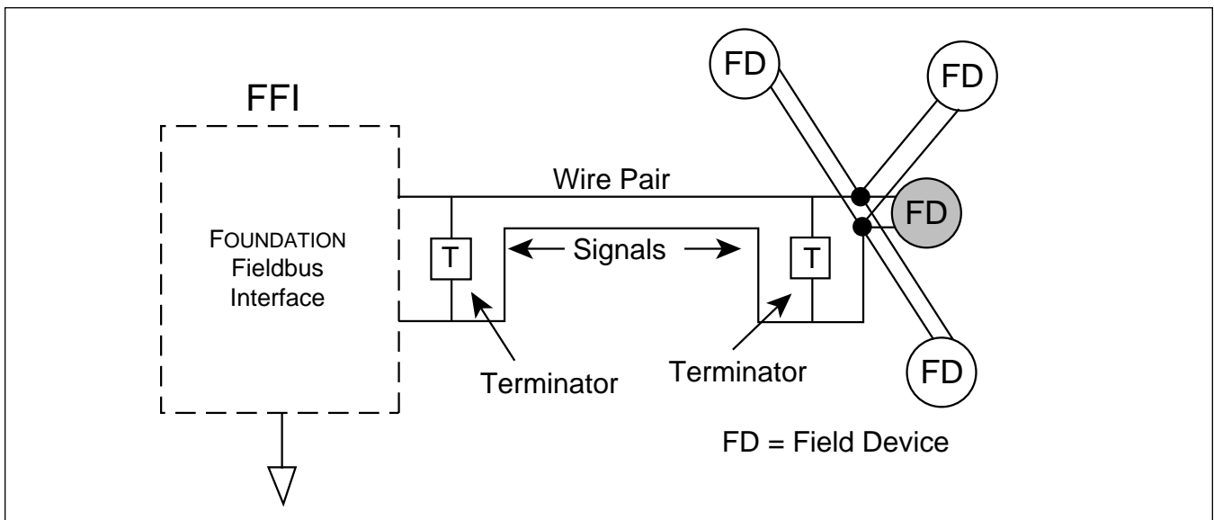
Figure 4.1-3 Fieldbus Network With Additional Devices Added
