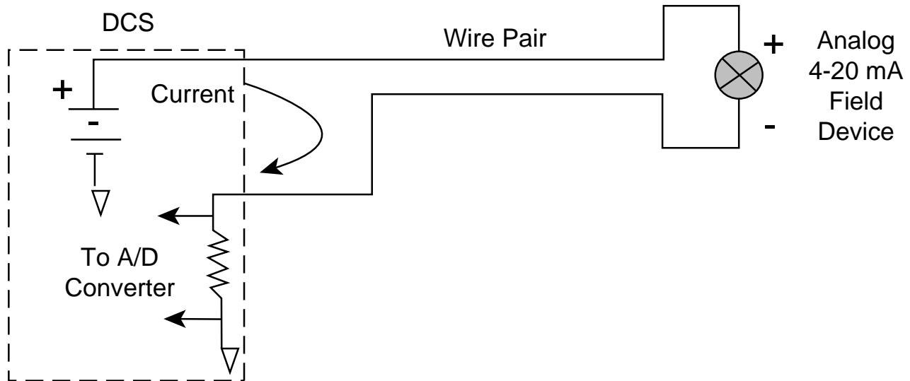
Figure 4.1-1 4-20 mA Current Loop Connection
