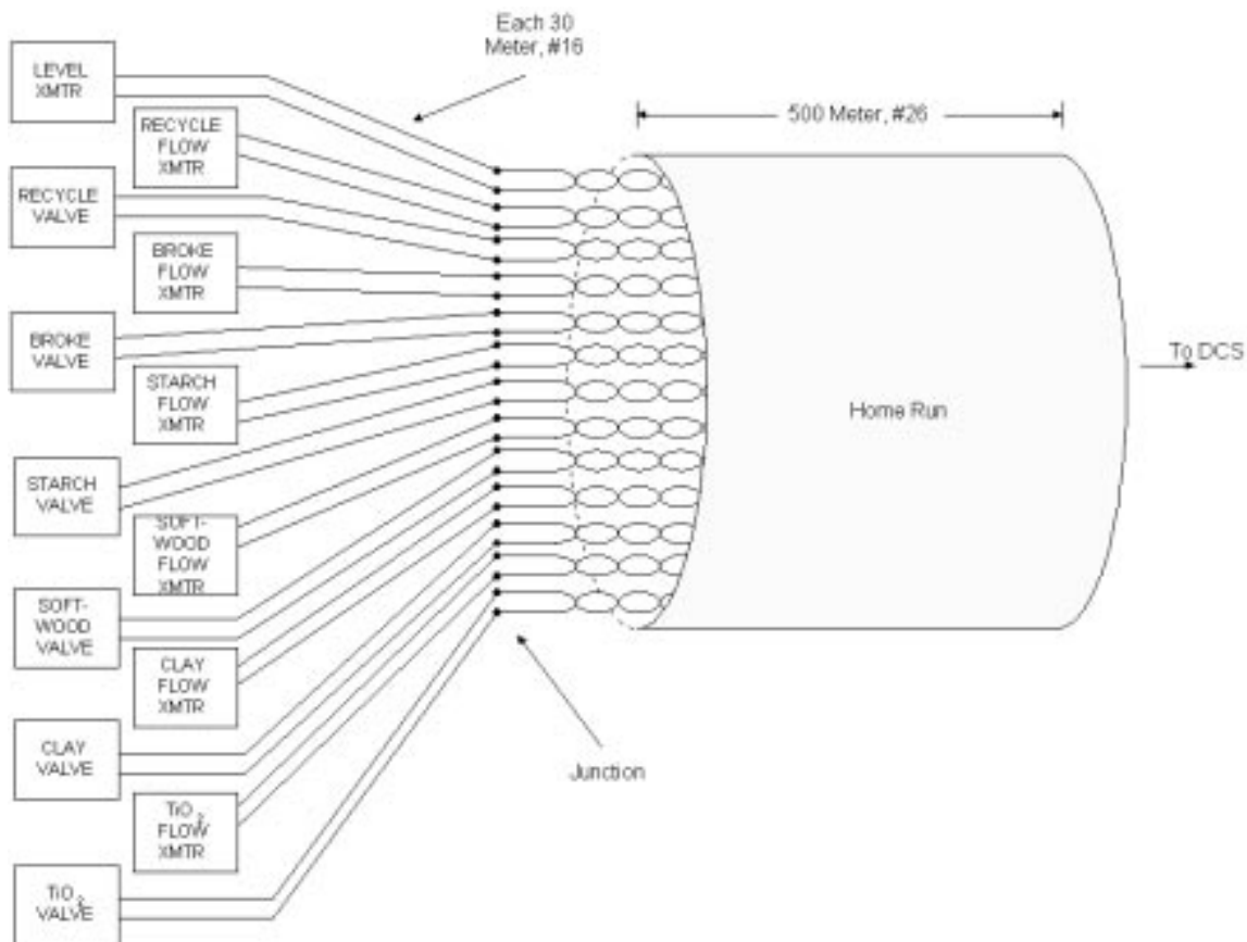
Figure 7.2-3 Original Wiring Diagram for Paper Mill Example
