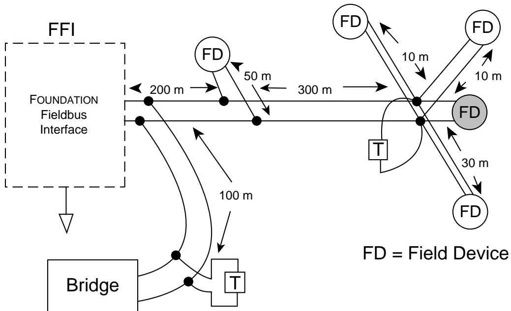
Figure 4.2-2 Segment Lengths for New Fieldbus Network
