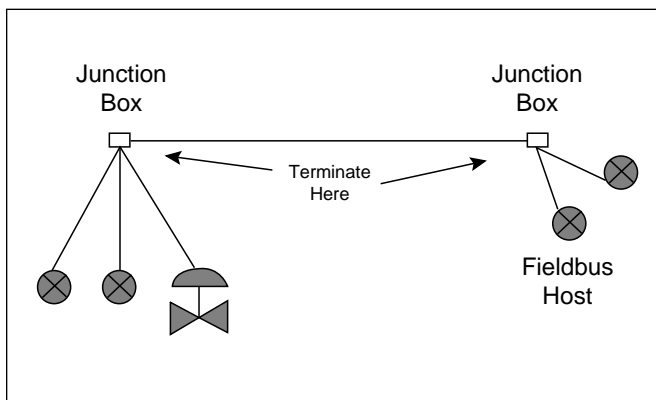
Figure 5.4-1 Tree Topology
