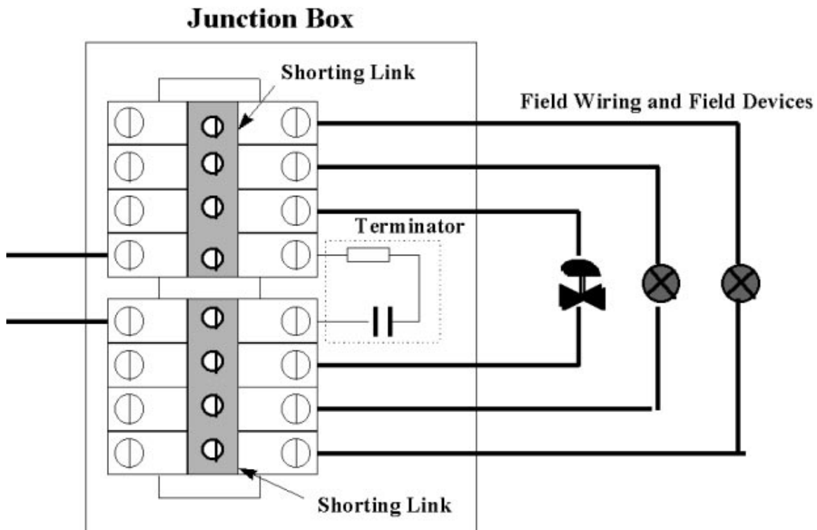
Figure 6.2-1 Terminal Block in Field Mounted Junction Box
